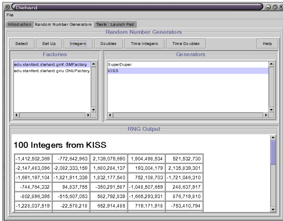
Figure 1: JDiehard GUI
