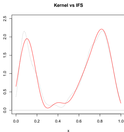
Figure 2: Old Faithful geyser data rescaled on [0,1] . Dotted line is the kernel estimator (bw=0.03, kernel=Gaussian), solid line is the IFS-Fourier expansion estimator (iterated 2 times, 26 Fourier coefficients).
