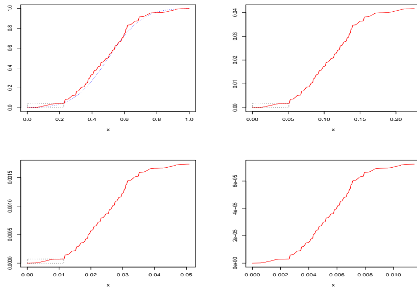
Figure 1: The fractal nature of the (quantile) IFS distribution function estimator. The dotted line is the underlying truncated Gaussian distribution. The dotted rectangle is to represent the area zoomed in the next plot (left to right, up to down). The dotted boxes are in the order: [0, \hat{q}_2] \times [0, \hat{q}_2] , [0, \hat{q}_2^2] \times [0, \hat{q}_2^2] and [0, \hat{q}_2^3] \times [0, \hat{q}_2^3] .
